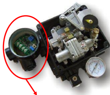
Retransmissor / Position Transmitter
